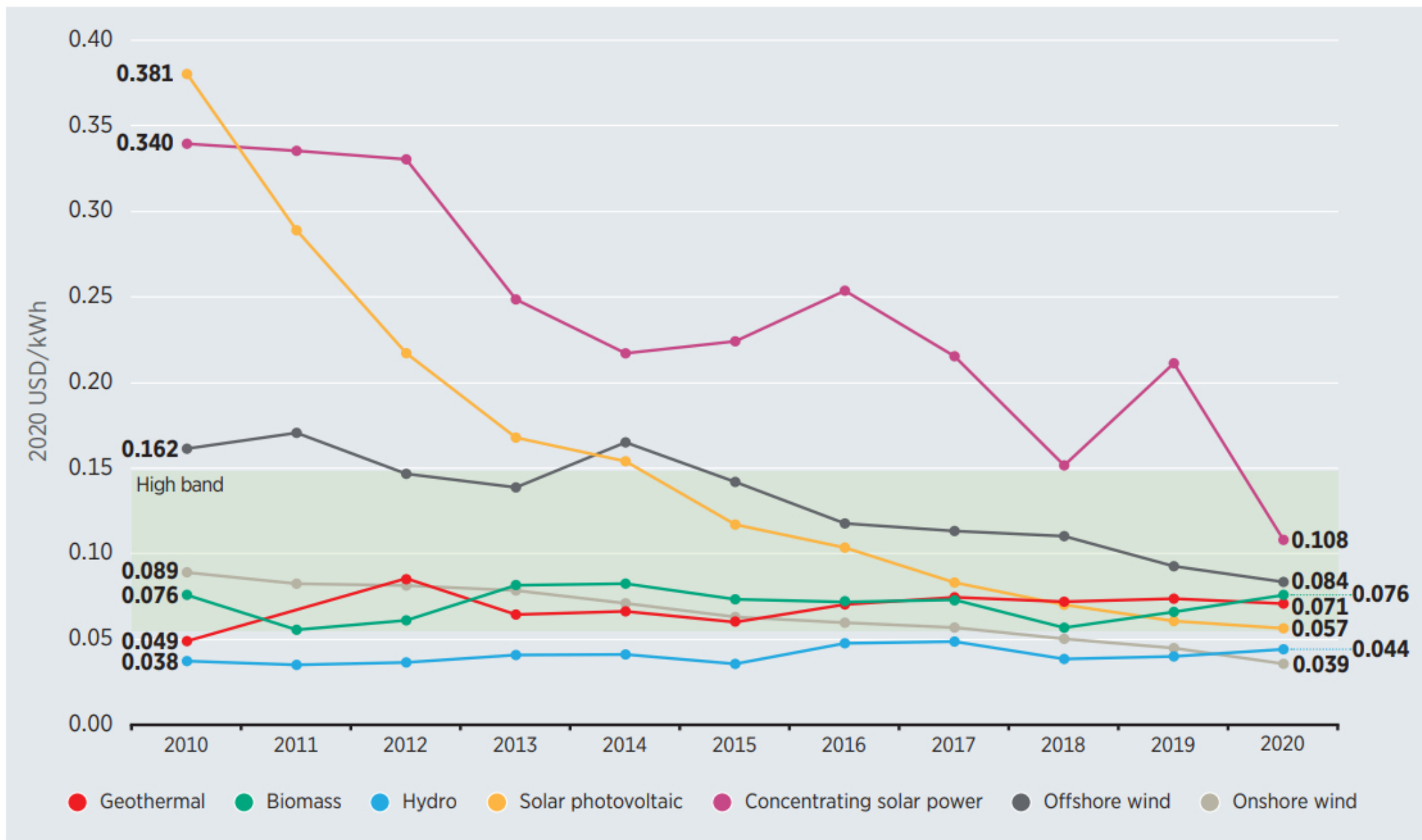
Figure 1.6 Global weighted-average utility-scale LCOE by technology, 2010-2020
