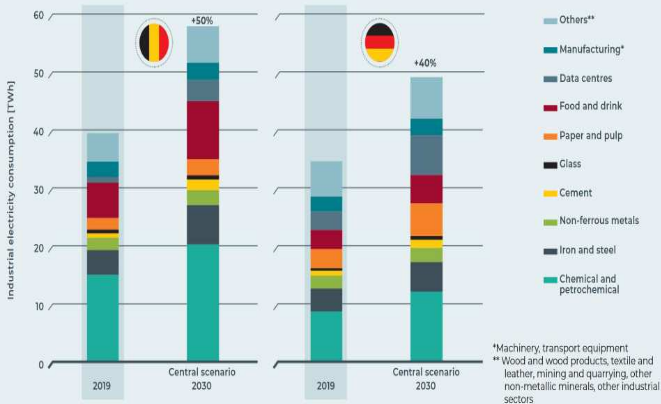
FIGURE 4 – EVOLUTION OF THE ANNUAL ELECTRICITY CONSUMPTION IN BELGIUM AND THE 50HERTZ AREA IN THE LEAD-UP TO 2030
